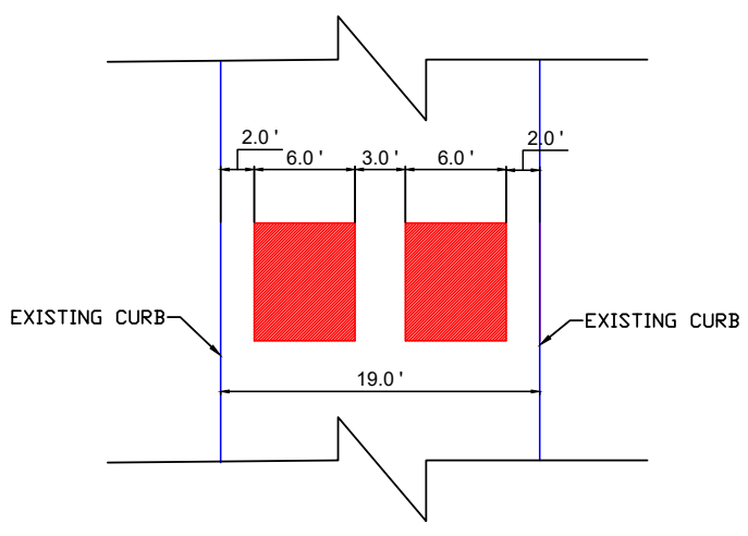
PROPOSED SPEED CUSHION DETAILS NTS
