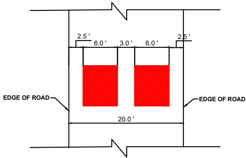
PROPOSED SPEED CUSHION DETAILS
