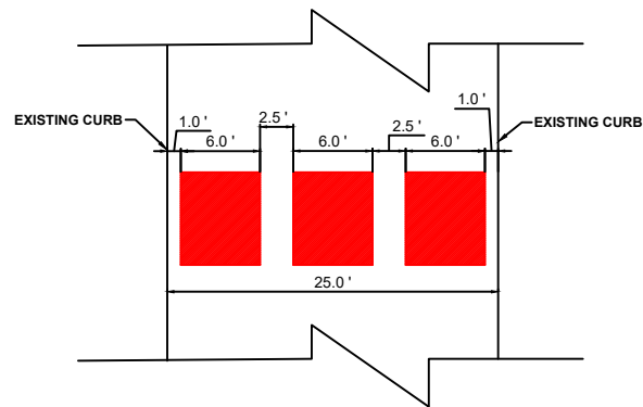
PROPOSED SPEED CUSHION DETAILS NTS
