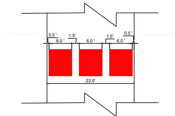
PROPOSED SPEED CUSHION DETAILS NTS
