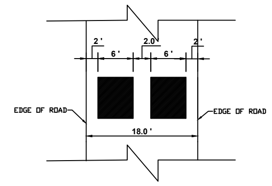
PROPOSED SPEED CUSHION DETAILS NTS
