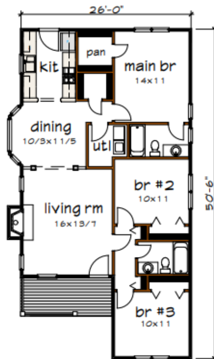
Floor 1 plan
