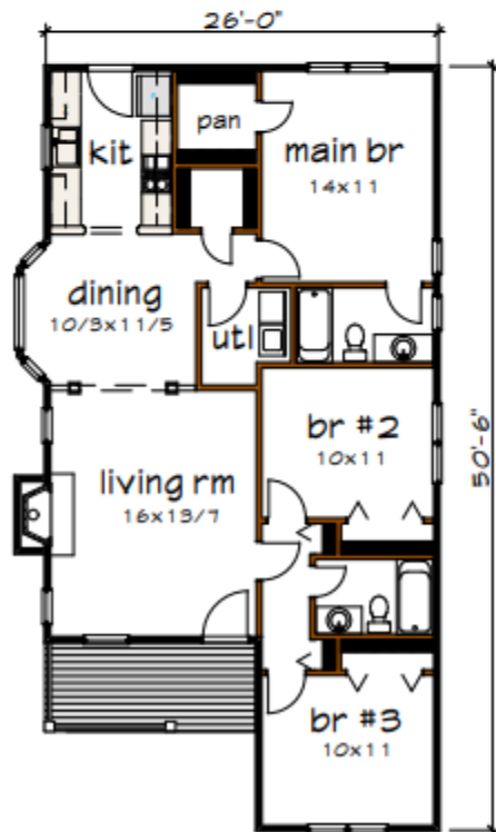
Floor 1 plan
