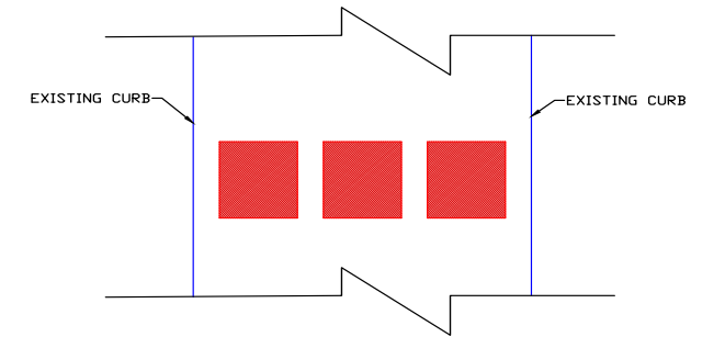
PROPOSED SPEED CUSHION DETAILS NTS
